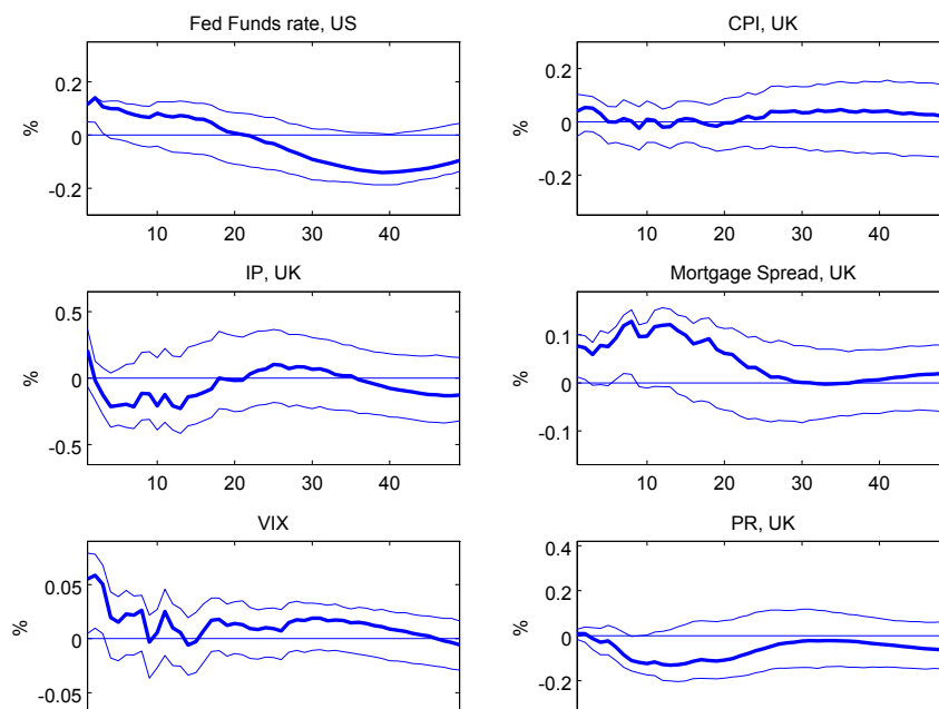
Figure 7: Response of the UK (% points) to a 20bp increase in the US one year rate(HF instruments of Gertler and Karadi(2014))
