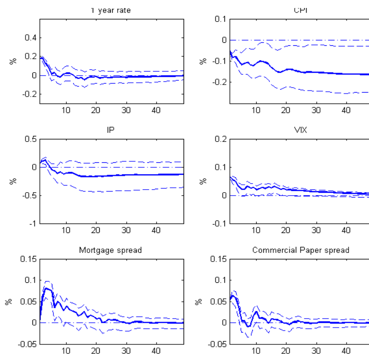
Figure 6: Response of the VIX to a 20bp increase in the US one year rate. Instruments from Gertler and Karadi(2014)
