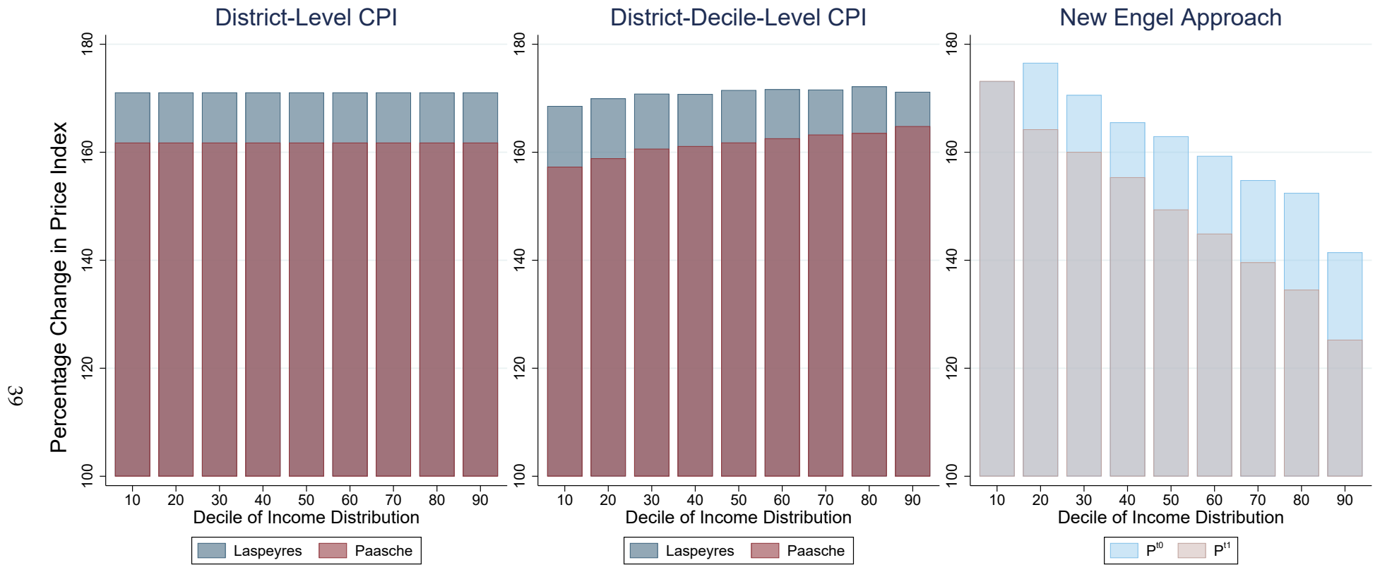
Figure 5: Indian Cost of Living Inflation 1987/88-1999/2000: New Engel Approach Compared to Existing CPI Estimates
