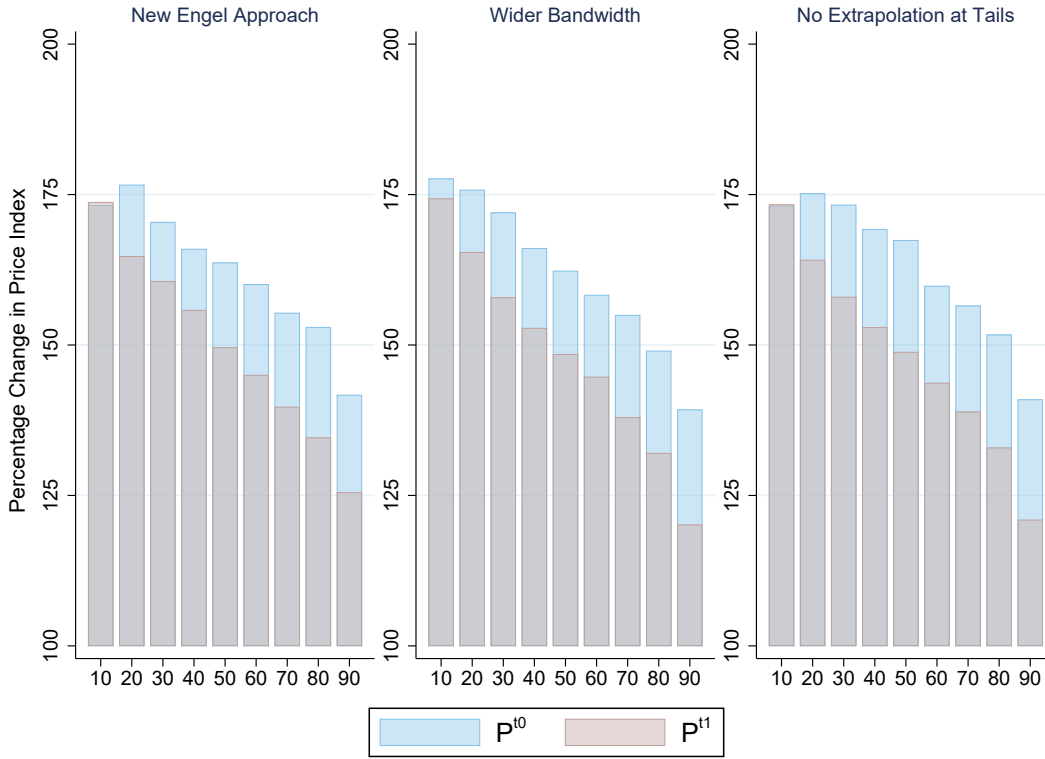
Figure A.7: Alternative Estimates of Relative Engel Curves
