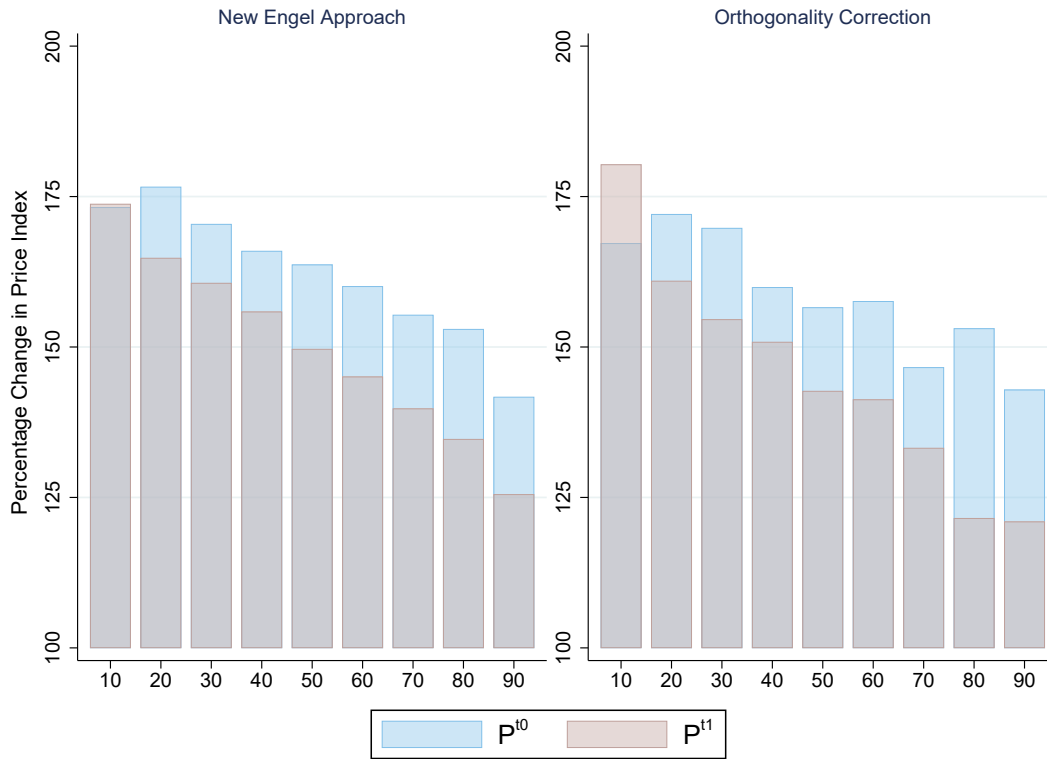
Figure A.5: Applying Orthogonality Correction for Confounding Price Effects ( \sigma = 4 )
