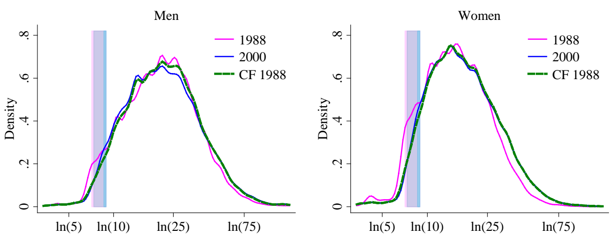
Figure 11. Counterfactual Densities 1988-2000
