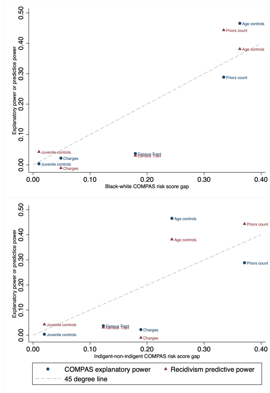
Figure 4: Contribution of components to overall explanatory and predictive power vs. black-white risk score gap and indigent-non-indigent risk score gap (using census tract-level variables)
