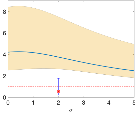
Figure 7: Ratio of \text{std}(\sigma(\Delta c_t - \Delta c_t^*) - \Delta q_t) after/during the Bretton Woods System
